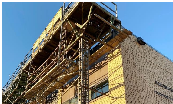
Recently completed work at the Neigebaur Administration Building Renovation. Pictures show new wall framing and façade restoration.
